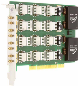
1 to 4 channel PCI (4 channel version shown) for arbitrary waveform generator card series: M2i.60xx/61xx, M2i.60xx/61xx-exp and MI.60xx
