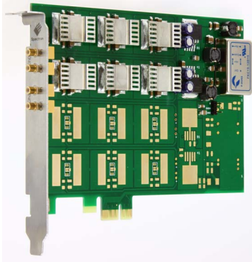
1 to 4 channel PCIe x1 (2 ch version shown) for arbitrary waveform generator card series: M2i.60xx/61xx, M2i.60xx/61xx-exp and MI.60xx
